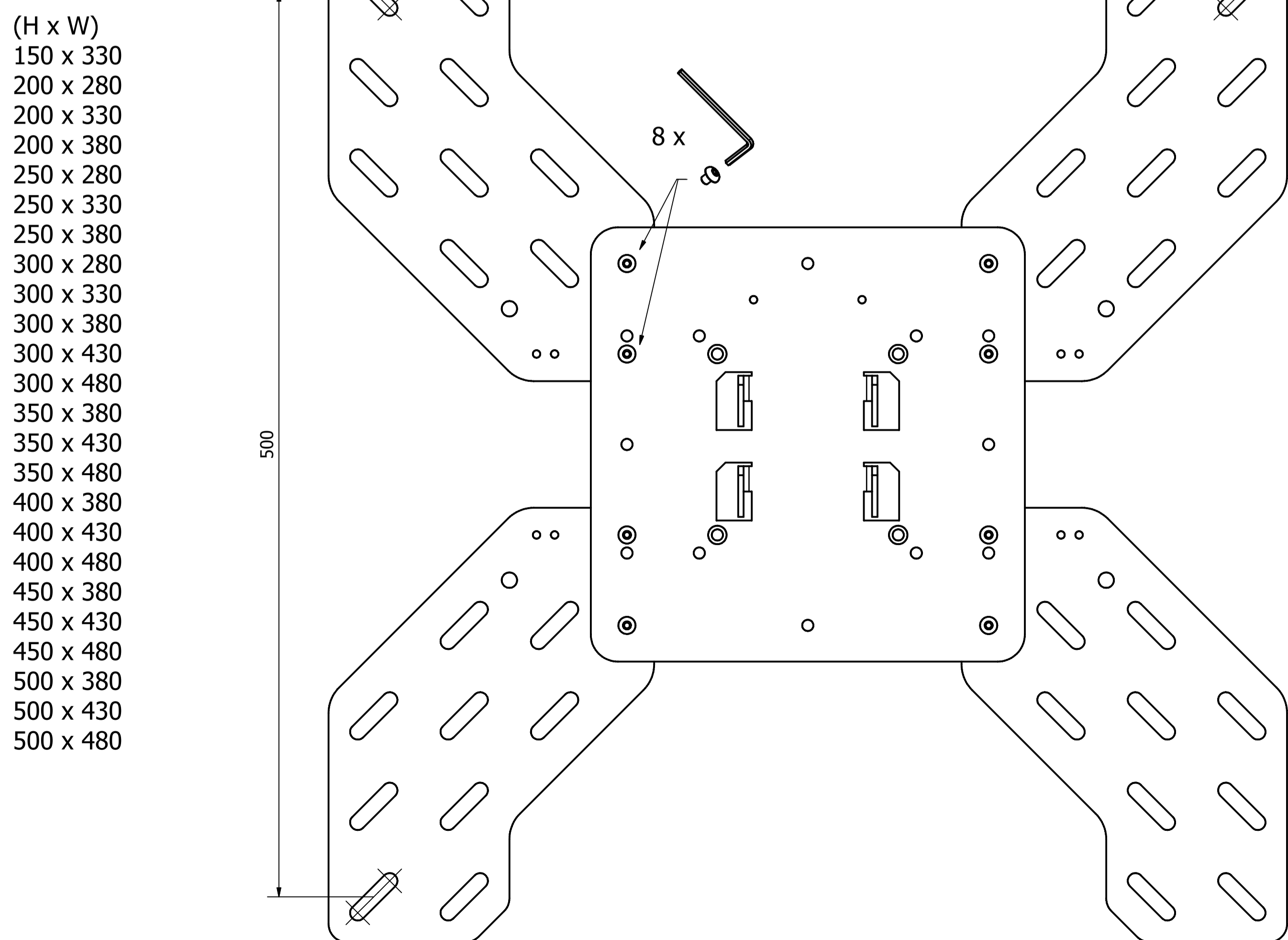
Assembly variant 3
