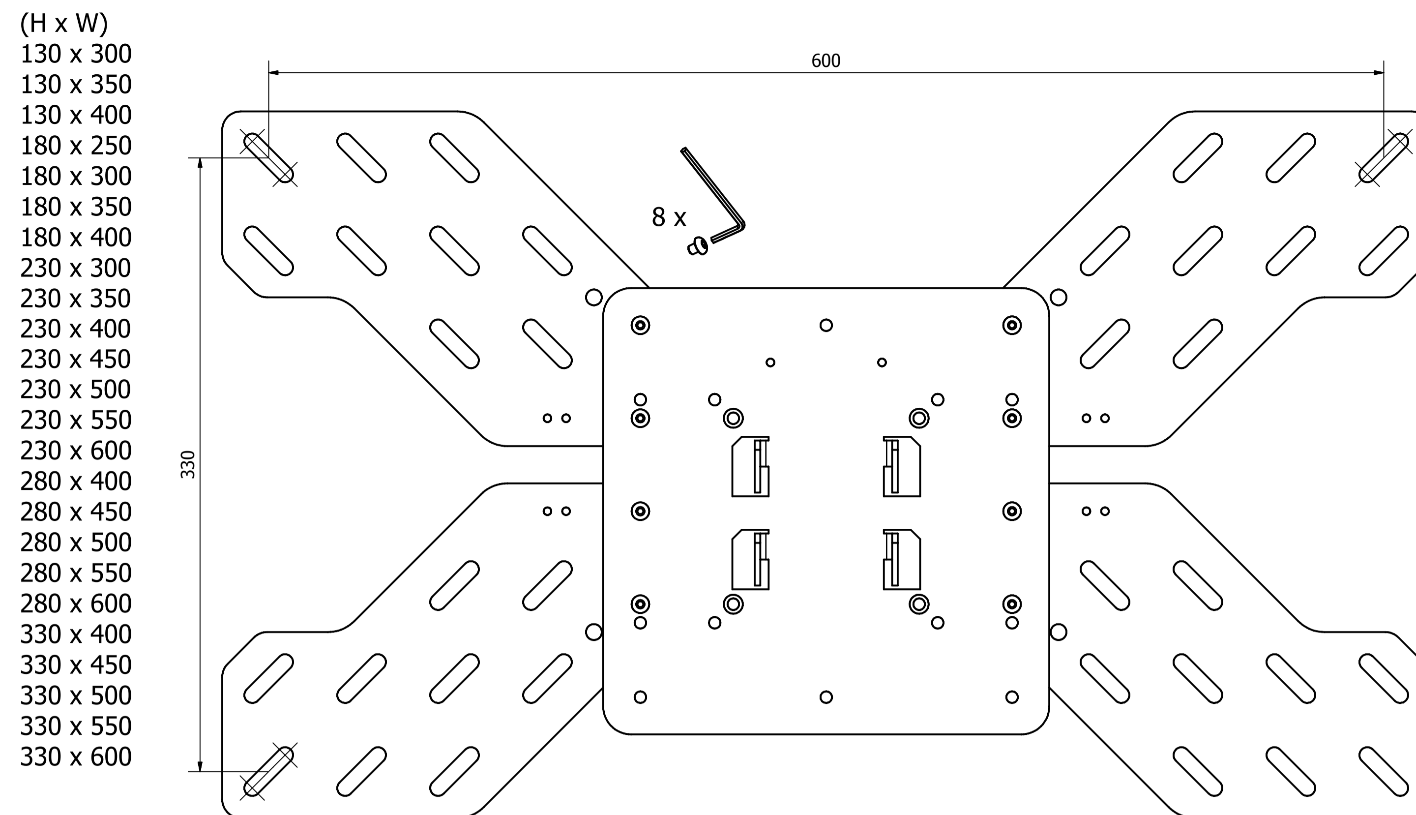
Assembly variant 2
