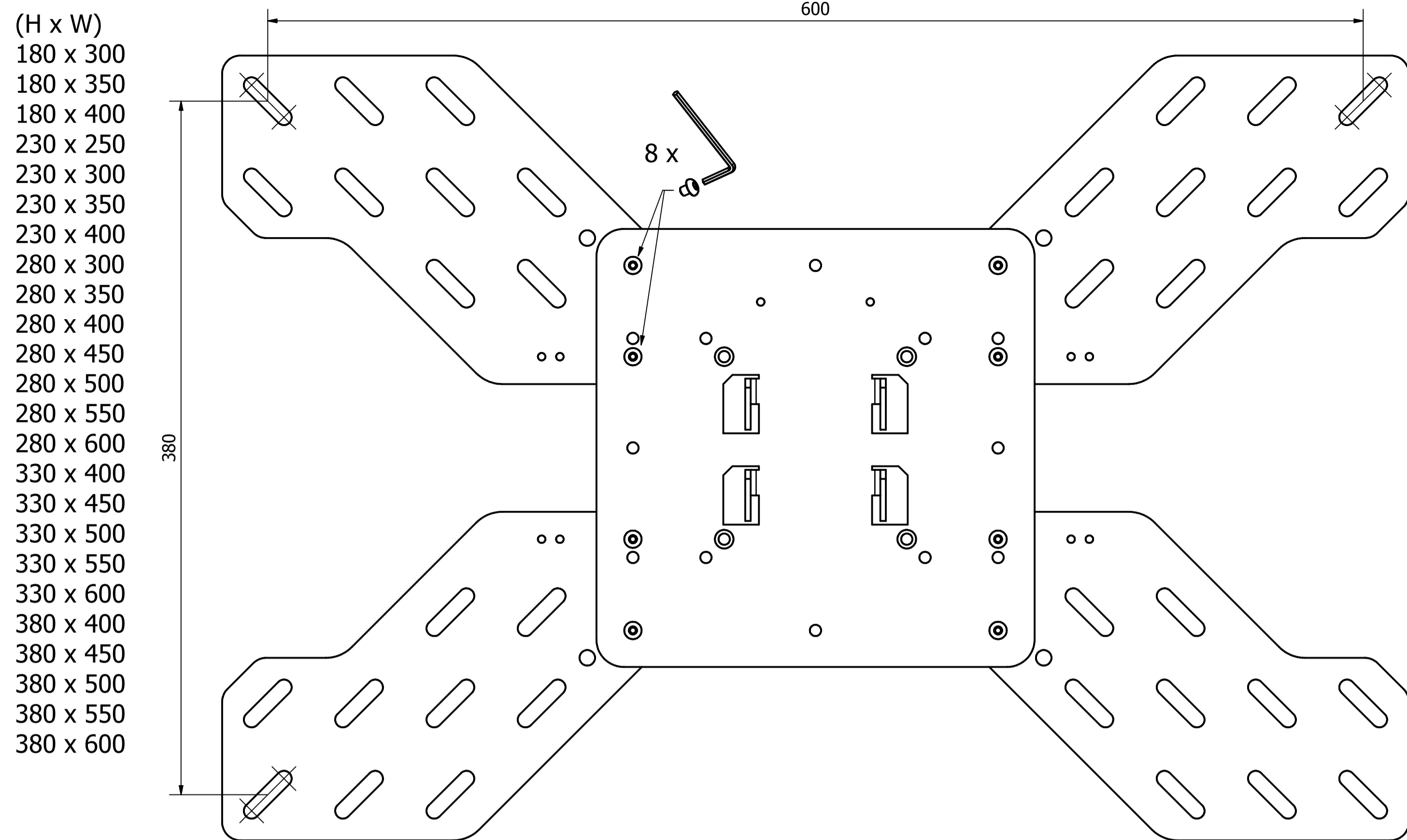
Assembly variant 1
