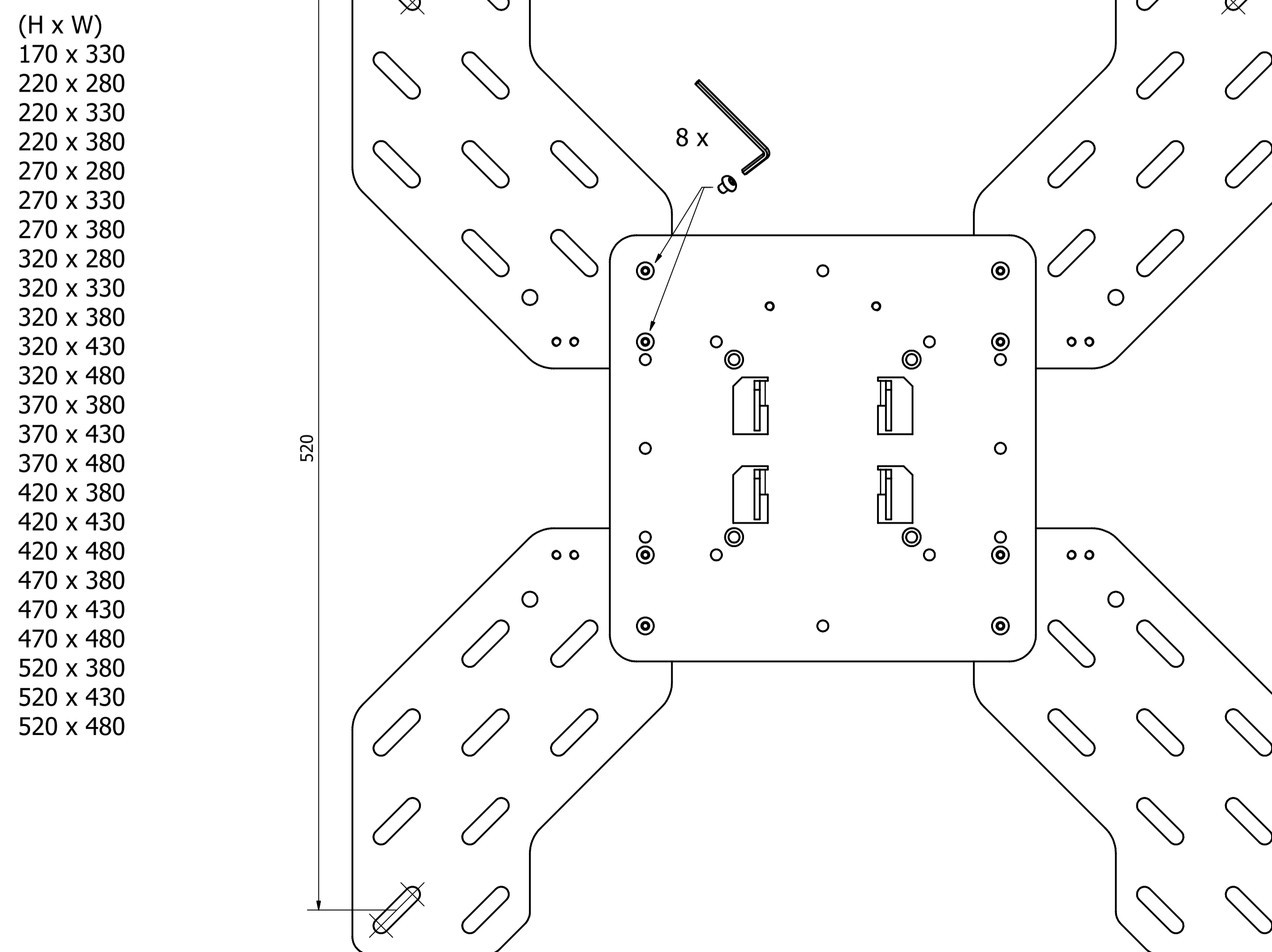
Assembly variant 4
